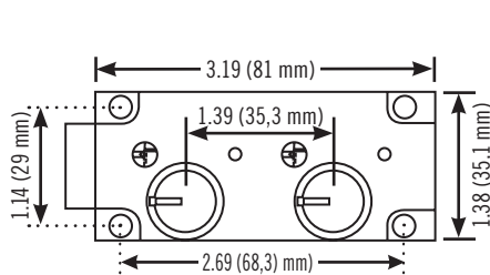
4420—designed for matchwork to all Corbin guard keys (RH model shown here)
